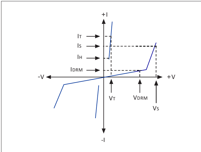
V-I Characteristics
